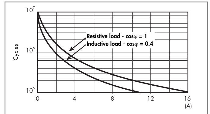
F 46 - Electrical life (AC) v contact current
